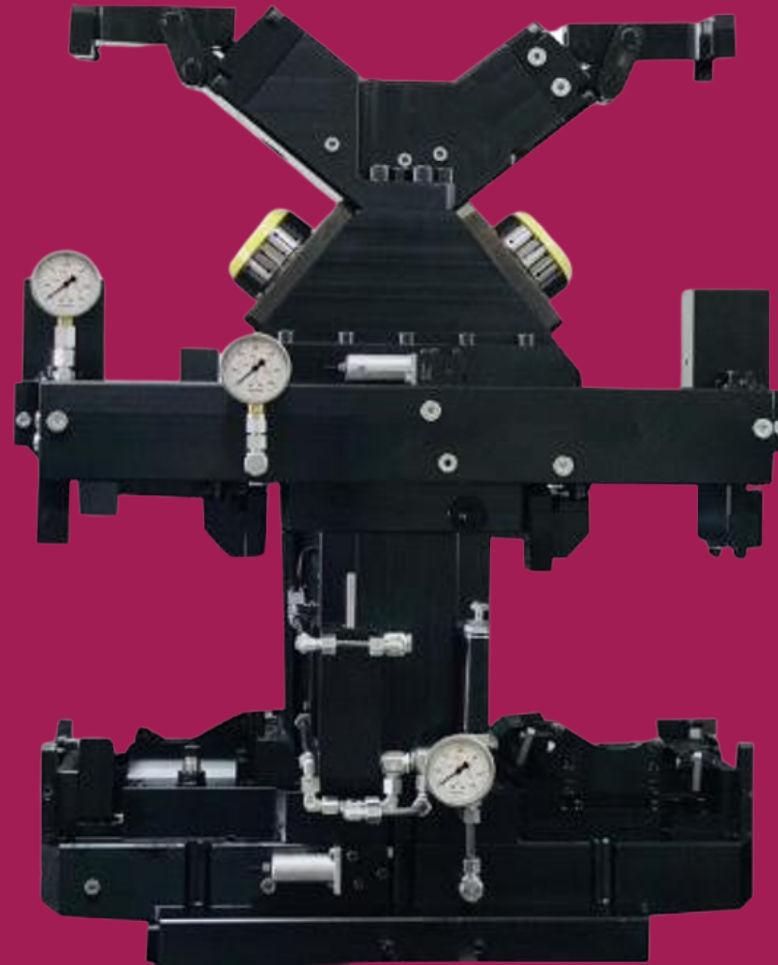
HORIZONTAL MACHINING FIXTURE
